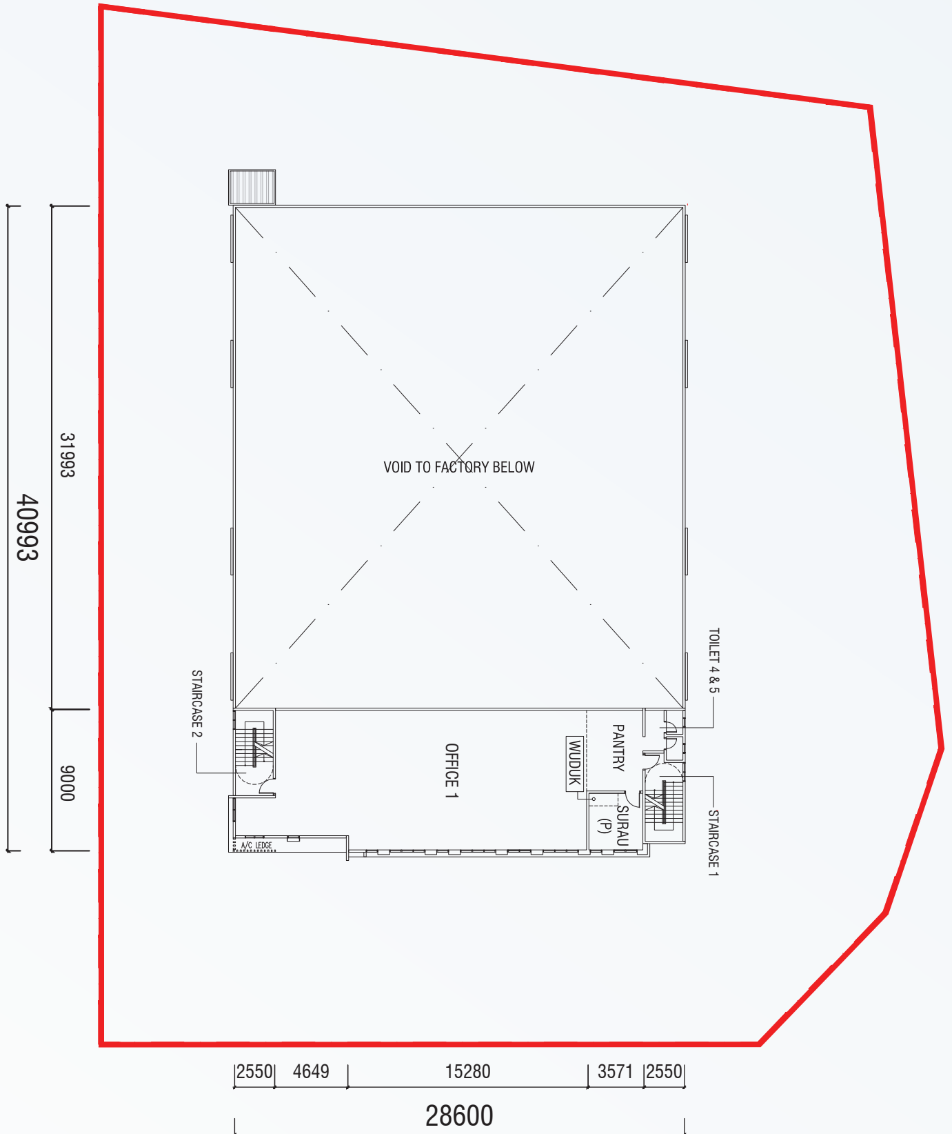
FIRST FLOOR
